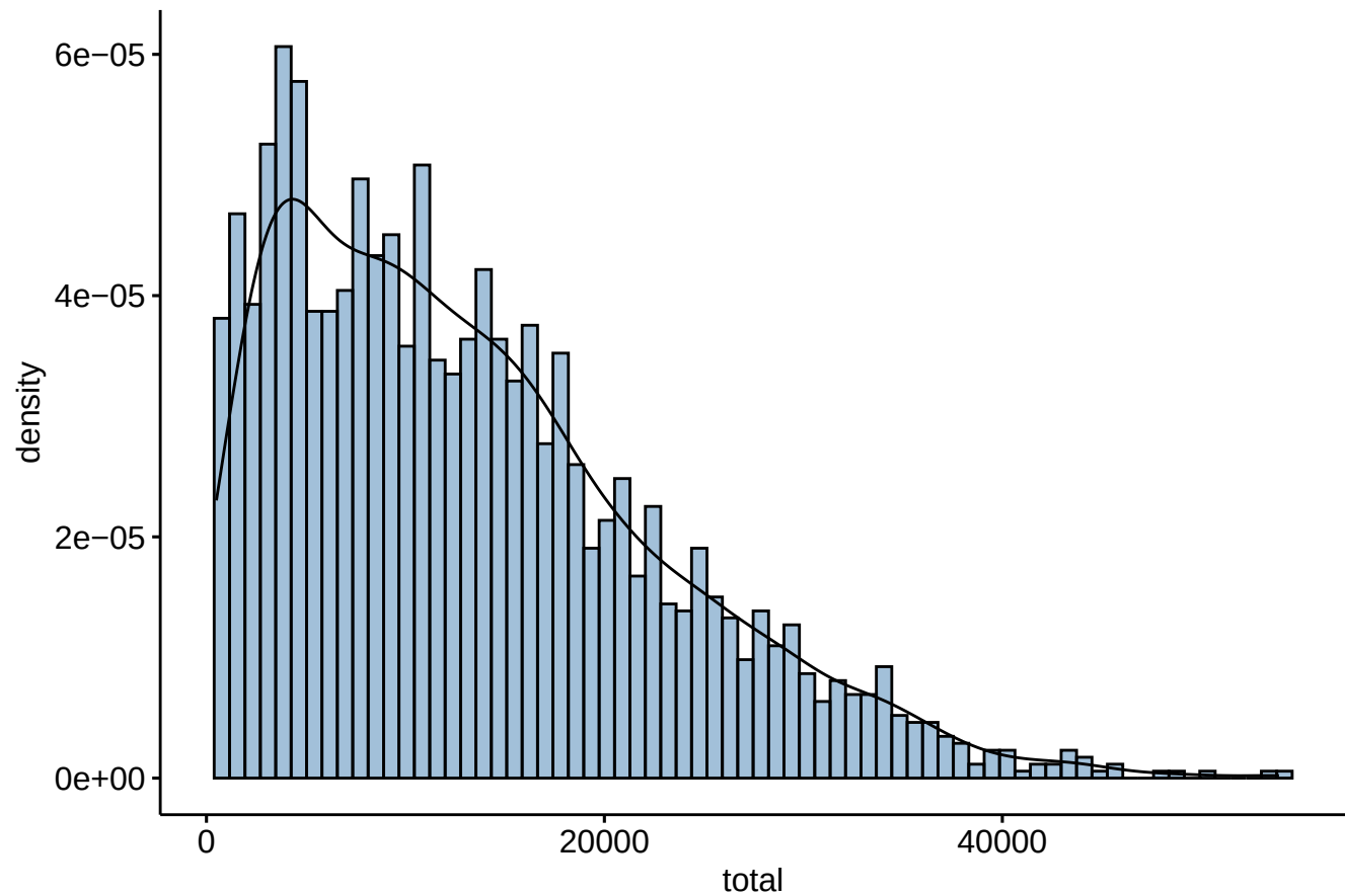
Cluster 12
